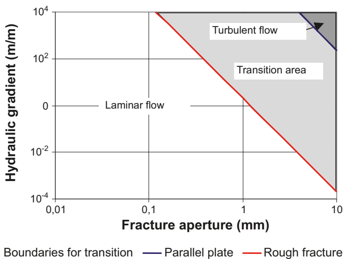
Figure 4-9. Transition from laminar to turbulent flow in fractures of different apertures and hydraulic gradients. Modified from /Gustafson 2010/.
